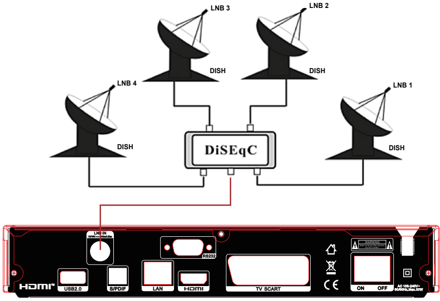
Figure7. Connecting to Dish LNB
