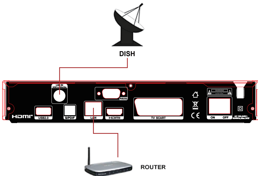
Figure6. Connecting to Dish LNB
